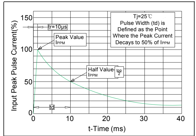
FIG.2: Pulse Waveform
