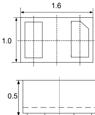
Package Dimensions (mm) Circuit and Pin Schematic
