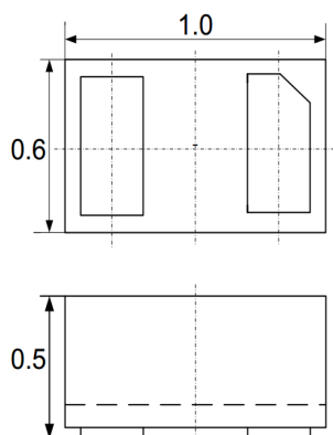
Package Dimensions
