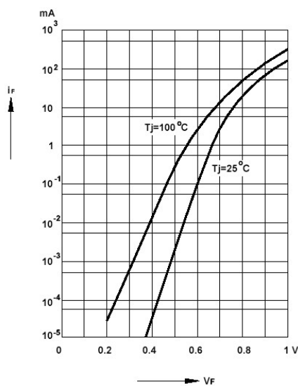
Forward characteristics
