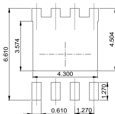
DIMENSIONS: MILLIMETERS
